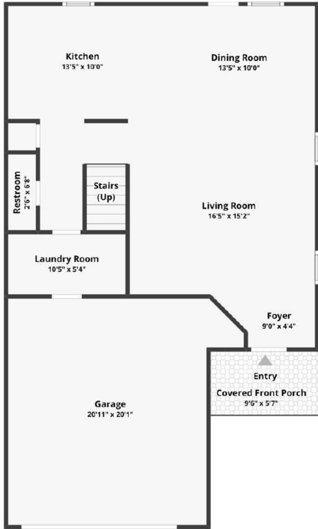
FLOOR 1
